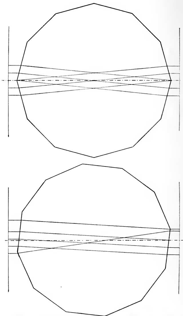
FIG. 4. ( Upper ) Position of the rotating prism, two edges on the optical axis.
